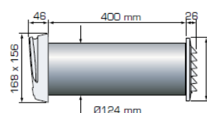
Measurement TL80F-dBS
