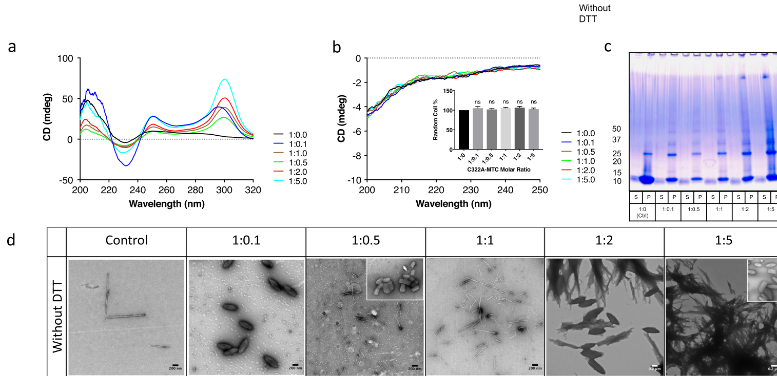
Fig. 4. Inhibition of assembly of dGAE-C322A in non-reducing conditions. C322A variant (100 \mu M) was incubated with MT using different molar ratios in the absence of 10 mM DTT in 10 mM phosphate buffer (pH 7.4) for 24 h at 37 ^{\circ} C and with 700 oscillations per minute of agitation in the dark. After 24-h incubation, the samples were centrifuged for 15 min at 4 ^{\circ} C and 20,000g. The CD spectra were recorded for both (a) pellet and (b) supernatant; inset shows a graphical representation of relative intensity at 200 nm against dGAE/MT ratio where 1:0 intensity is 100%. (c) Coomassie blue-stained, non-reducing SDS-PAGE gel of separated supernatant (S) and pellet (P) fractions of dGAE (100 \mu M) incubated with different ratios of dGAE/MT as shown. (d) Transmission electron micrographs of negatively stained dGAE (100 \mu M) incubated for 24 h at 37 ^{\circ} C with MT at different molar ratios for dGAE/MT, in the absence of DTT from 0 h. The scale bars represent 200 nm.
